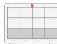
4 Size Drawer: Single Deep W 342 mm x H 52 mm x D 223 mm
